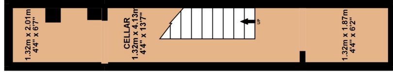
BASEMENT FLOOR 10.53 sq. m. ( 113.37 sq. ft. )
