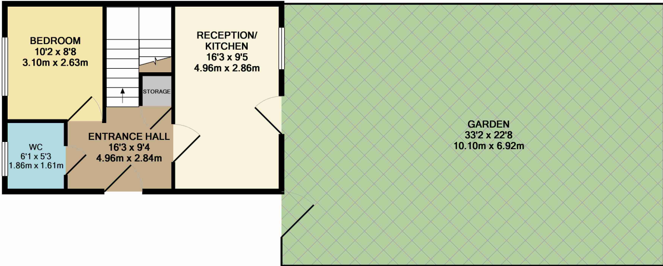
GROUND FLOOR APPROX. FLOOR AREA 390 SQ.FT. (36.3 SQ.M.)
